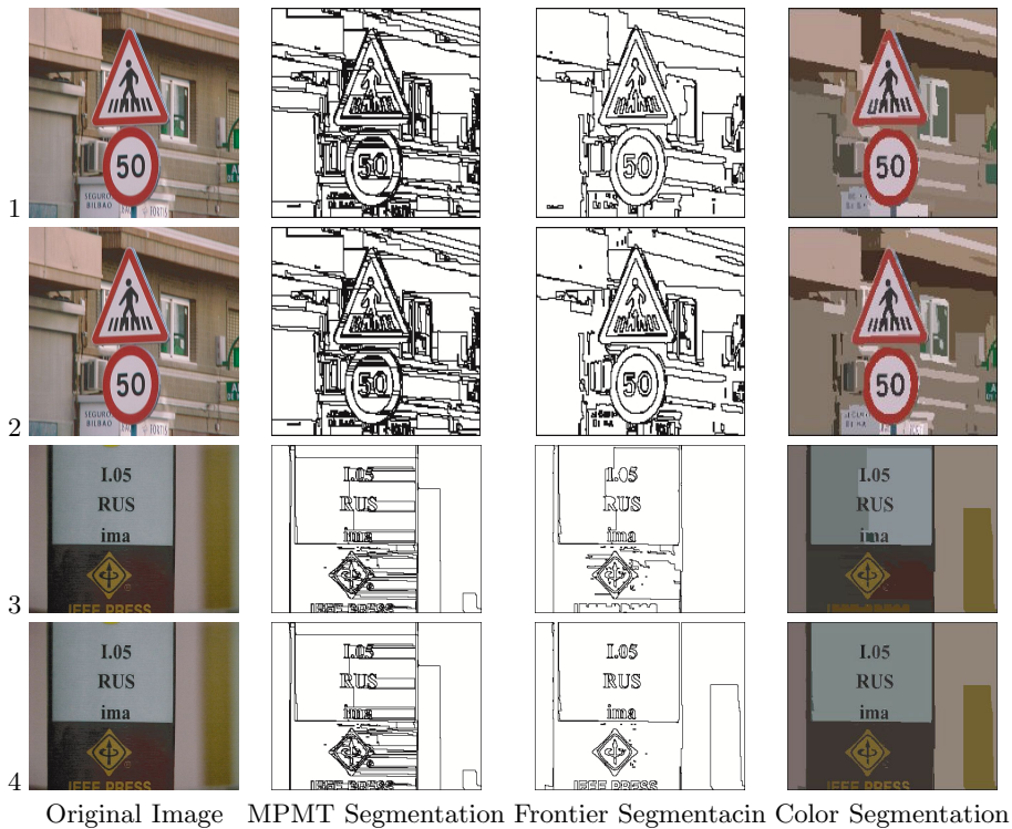
Fig. 4. Image Segmentation
