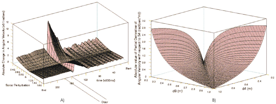
Fig. 5. (a) Change in angular velocity when sonar 9 is modulated with noise. (b) Representations of the absolute value of \partial\theta/\partial s_4 when s_4 = 0.33m .
