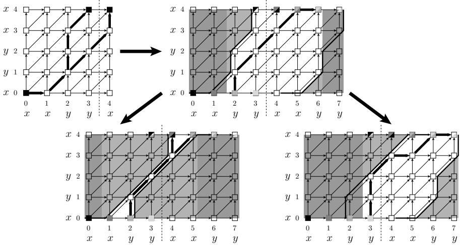
Fig. 6. Divide-and-Conquer procedure to compute the CDTW dissimilarity between [A = xxyy] and [B = xyyxx] . First, the optimal alignment between A and B and between Aa_0 and B is computed. The optimal path underlying the alignment between \sigma^0(A) and B (which is a displaced version of the optimal path between \sigma^4(A) and B ) is used as a frontier in the extended graph: only the white region must be explored to compute the optimal alignment between \sigma^2(A) and B and between \sigma^2(A)a_2 and B . The optimal path between \sigma^1(A) and B and \sigma^1(A)a_1 and B cannot cross the optimal path between \sigma^0(A) and B and between \sigma^2(A) and B . The optimal path between \sigma^3(A) and B and \sigma^3(A)a_3 and B cannot cross the optimal path between \sigma^2(A) and B and between \sigma^4(A) and B .
