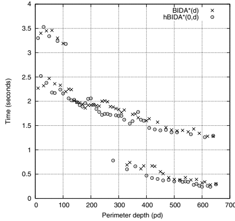
Fig. 3. BIDA^*_{p_d} vs. hBIDA^*_{0,p_d} in a 100 \times 100 maze
