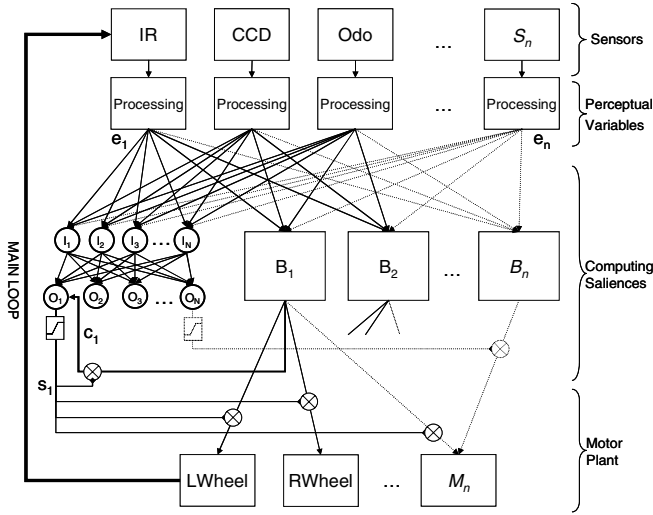
Fig. 3. Perceptual variables ( e_i ) form the input for the Saliency Neural Network. The output selection of the highest saliency ( s_j ) is gated to the motors of the Khepera. Notice the busy-status signal ( c_i ) from behavior B_1 to the output neuron.
