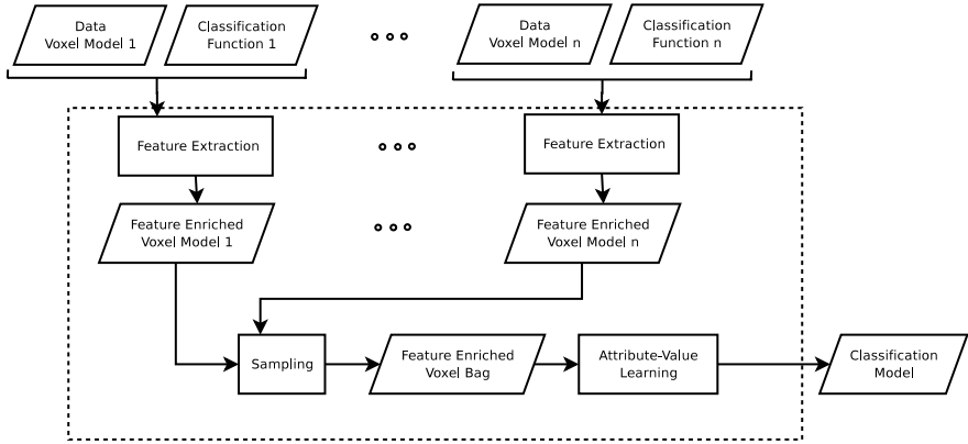
Fig. 2. The learning process adapted to use attribute value learning algorithms
