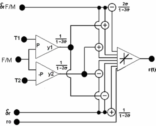
Fig. 4. Simplified neural structure of the recirculation control carried out by (5)
