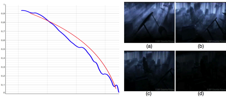
Fig. 4. Theoretical and real entropy series. \rho = 0.99038 .
