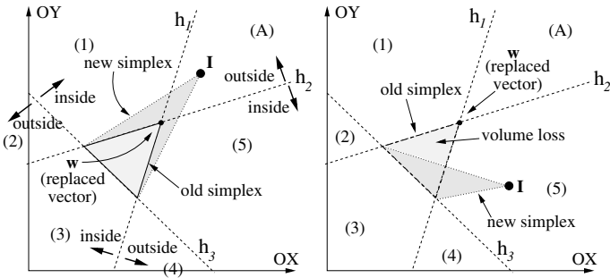
Fig. 2. Example of replacement of vector \mathbf{w} in \mathbb{R}^2 . Only patterns located in region A can replace \mathbf{w} (left panel). The replacement of \mathbf{w} by patterns situated in the remaining regions would reduce the simplex volume (right panel).
