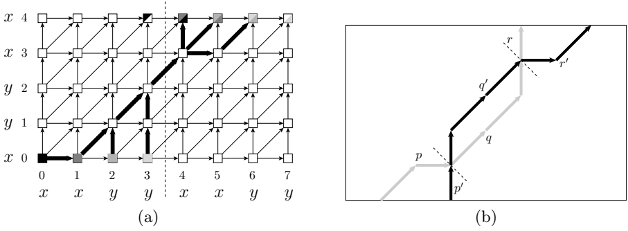
Fig. 5. (a) Extended warping graph for A = xxyy and B = xyyxx . The optimal alignment for [A] and [B] is the optimal path starting from some colored node in the lower row and ending at node with the same color in the upper row. The optimal path departing at (0, 0) is (0, 0), (1, 0), (2, 1), (3, 2), (4, 3), (4, 4) ; departing at (1, 0) : (1, 0), (2, 1), (3, 2), (4, 3), (4, 4) ; departing at (2, 0) : (2, 0), (2, 1), (3, 2), (4, 3), (5, 4) ; and departing at (3, 0) : (3, 0), (3, 1), (3, 2), (4, 3), (5, 3), (6, 4) . (b) Optimal crossing paths can be avoided: if the weight of the subpath q is greater than the weight of the subpath q' , the black path can be improved by traversing q' instead of q .
